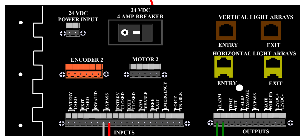
BA Bridge Plate Located on the "B" side of the turnstile
